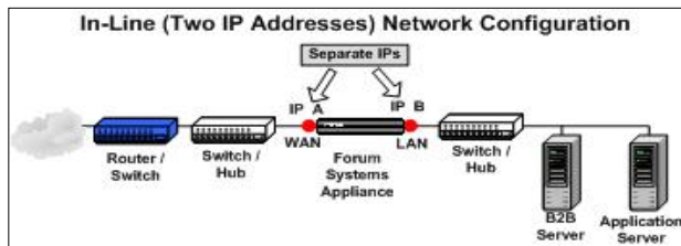
Figure 3: In-Line Configuration Schematic for Two IP Addresses.
