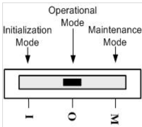
Figure 6: HSM Module Set to Operational Mode.
